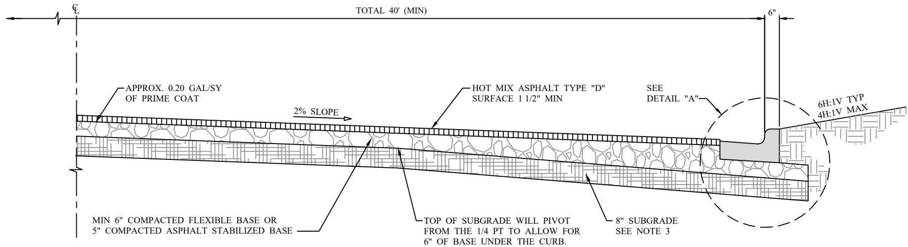
TYPICAL SECTION NOT TO SCALE
