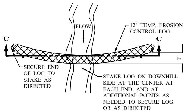
PLAN VIEW NOT TO SCALE
