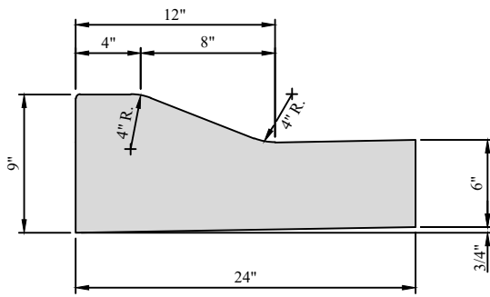
MOUNTABLE CURB NOT TO SCALE
