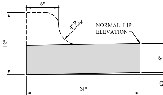
SIDE VIEW SAWTOOTH CURB NOT TO SCALE
