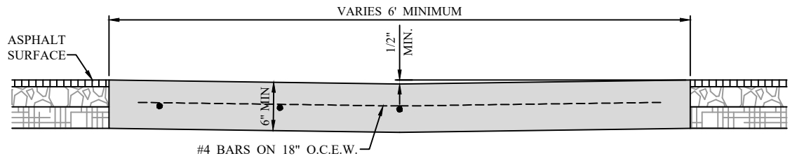
SECTION B - B VALLEY GUTTER DETAIL NOT TO SCALE
